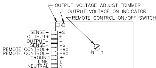
FIGURE 3. COMPONENT LOCATIONS
