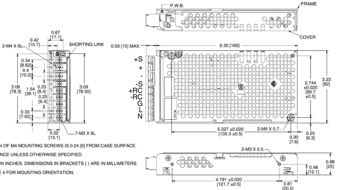
FIGURE 7. RTW 100W KC MODELS (WITH COVER) MECHANICAL OUTLINE DIAGRAM
