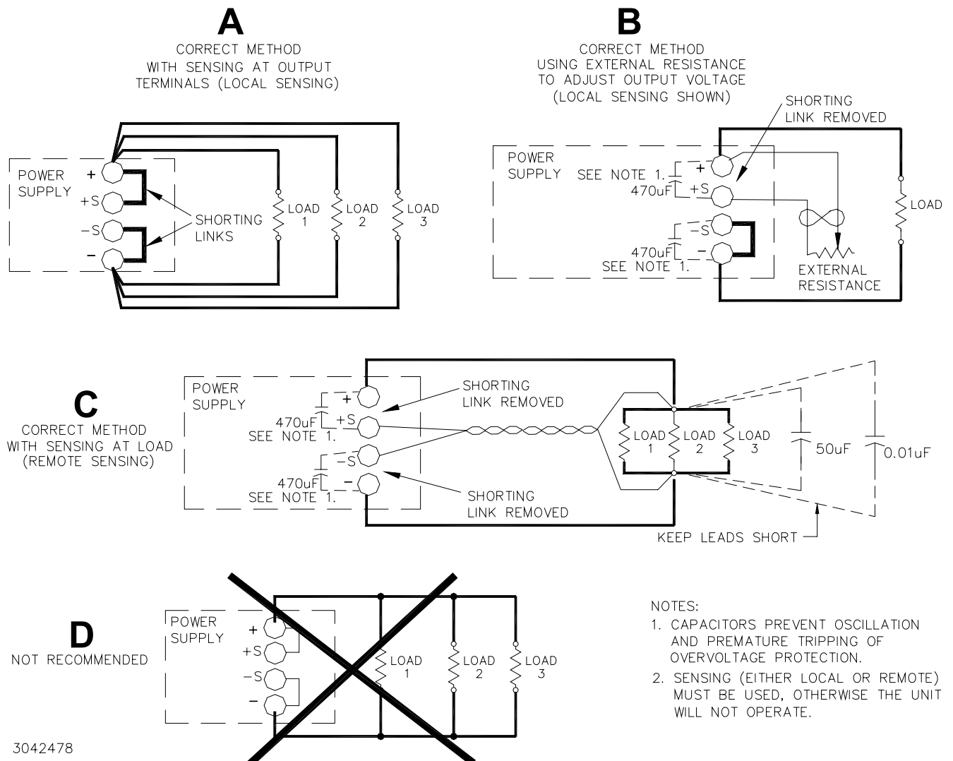
FIGURE 4. LOAD CONNECTIONS
